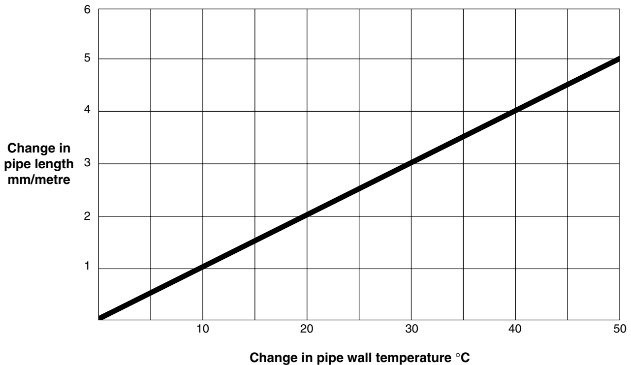
Expansion or contraction of pipe with temperature
